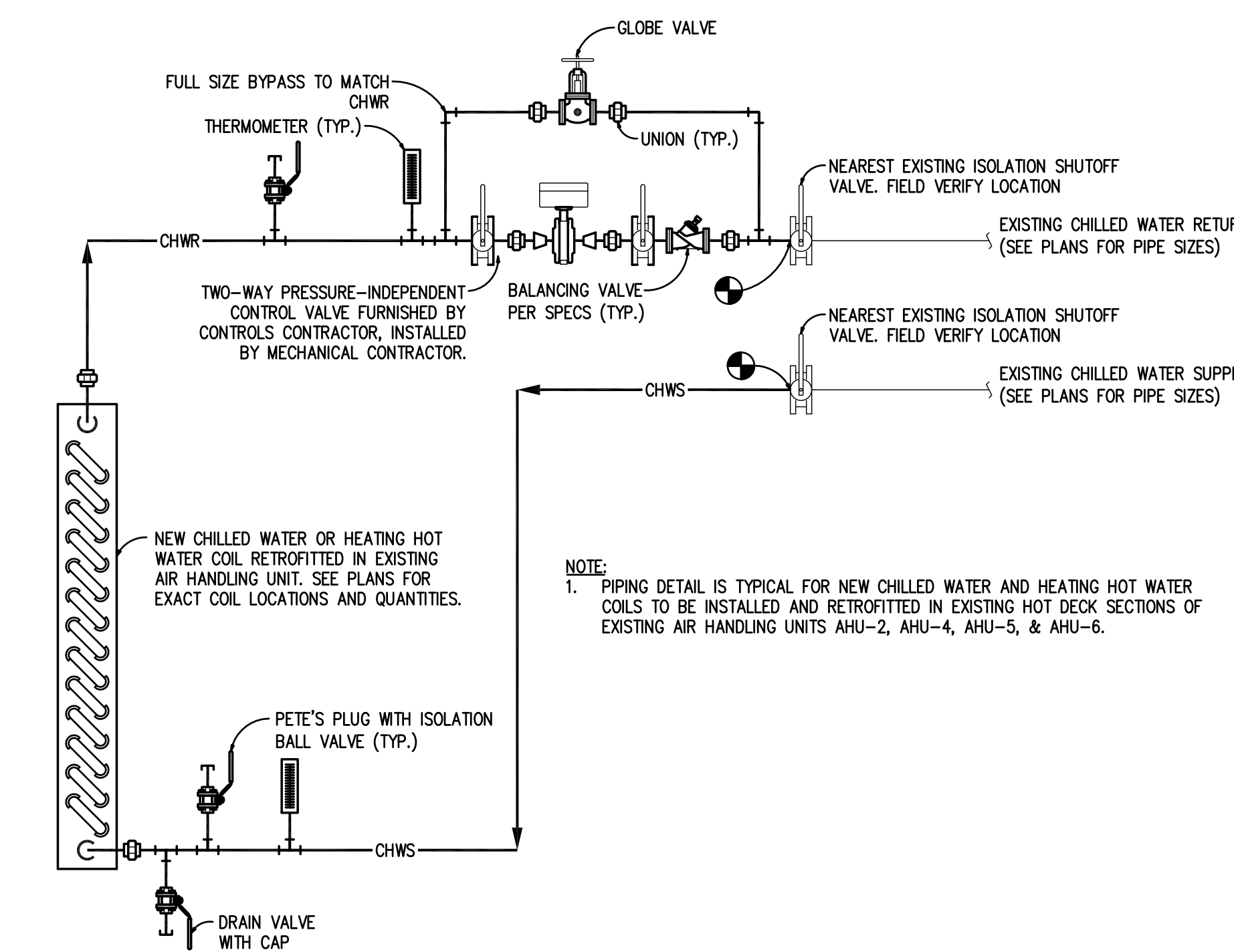
1 NEW TYPICAL WATER COIL PIPING DETAIL SCALE: N.T.S.
