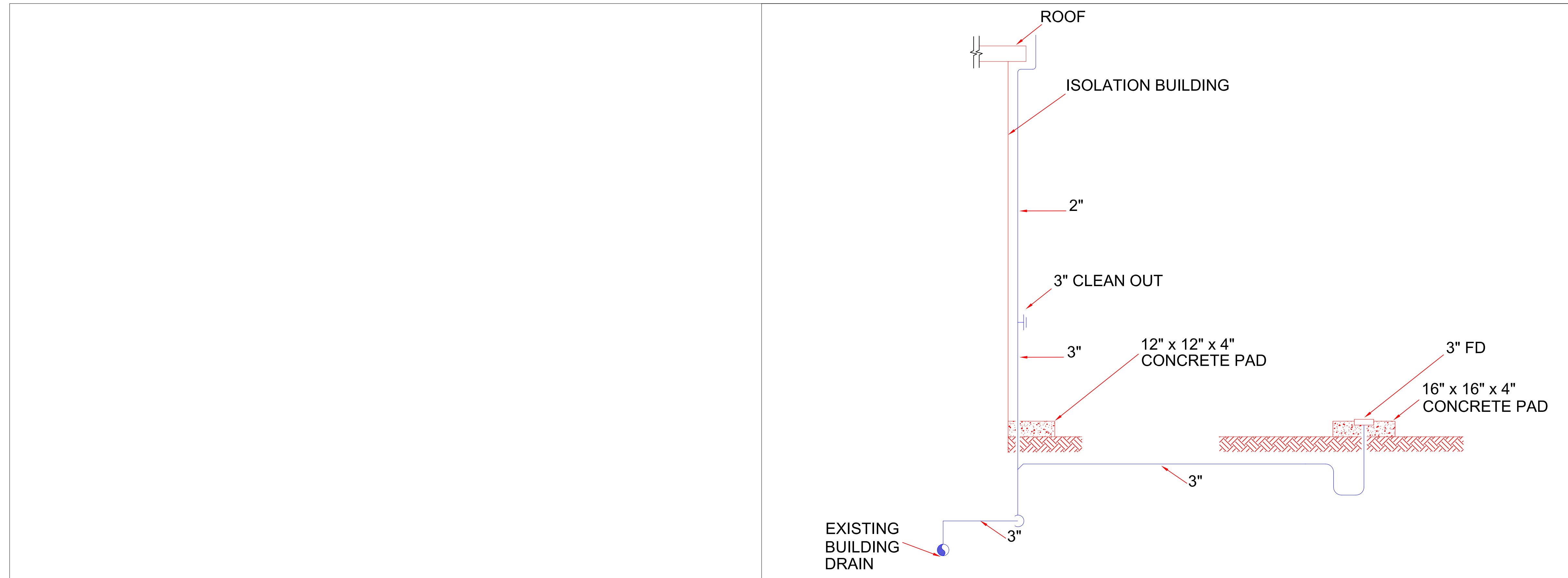
1-01 PLUMBING DETAIL ELEVATION NO SCALE
