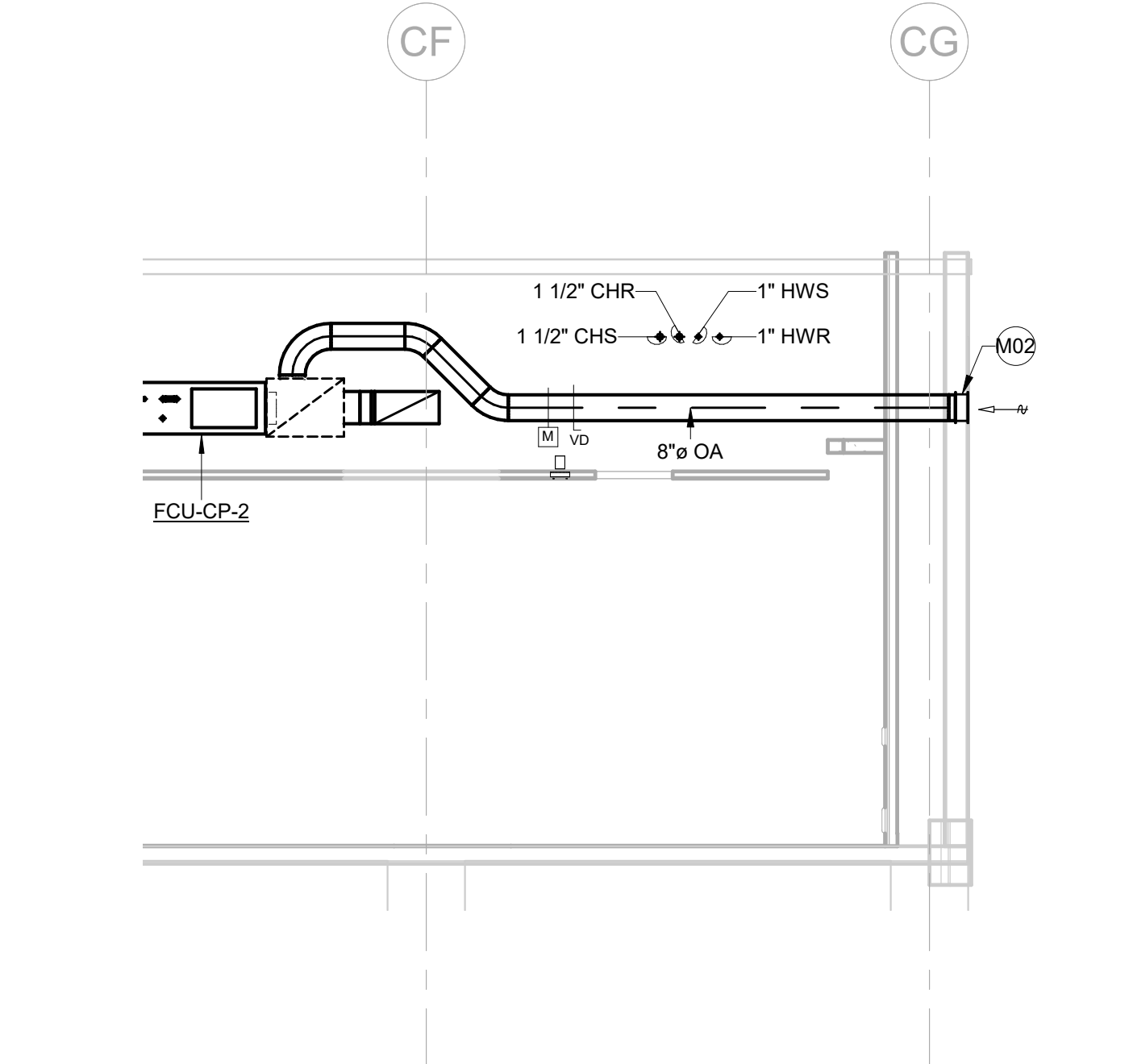
3 CENTRAL PLANT MECH SECTION 1/4" = 1'-0"
